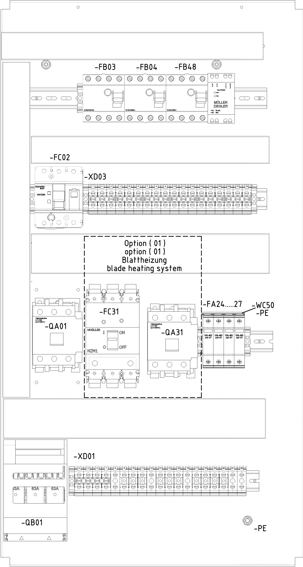
Montageplatte links unten mounting plate left below
